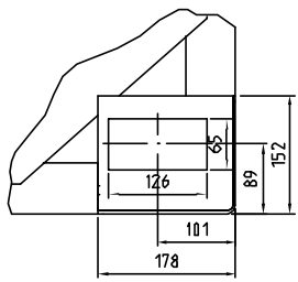
Detail D: (M 1:5)
